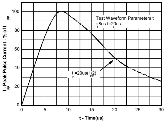
Pulse Waveform
